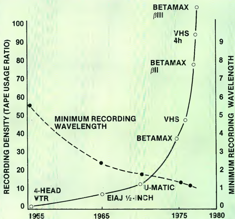
Figure 1. Shown are the improvement in videotape recording density with time and the improvement in minimum recording wavelength with time.
